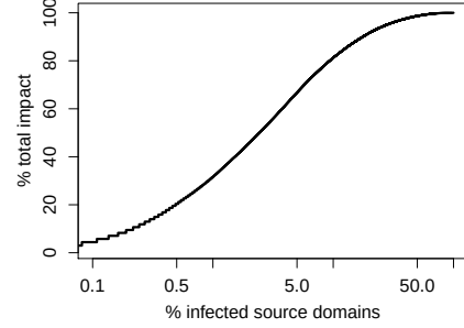
Figure 3: Rank-order CDF of domain impact reveals high concentration in search-redirection attacks.
