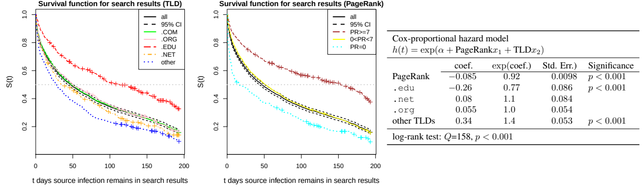
Figure 4: Survival analysis of search-redirection attacks shows that TLD and PageRank influence infection lifetimes.
